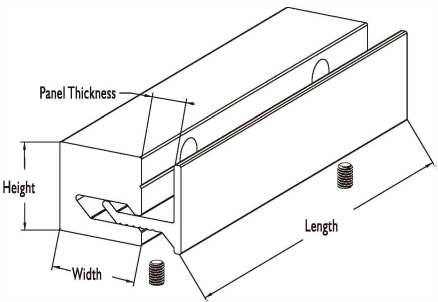
XCI7A+XCI7C KIT
